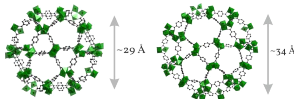
Figure 1. Two types of cages observed in Cr-MIL-101: dodecaedric cages containing five-membered rings (left) and hexacaidecaedric cages containing five-membered and six-membered rings (right). 17
