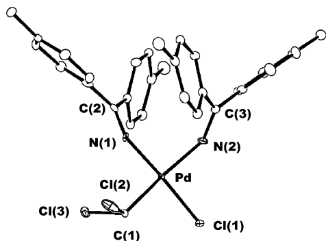
Figure 4. ORTEP drawing of 7 at the 30% ellipsoidal level. The hydrogen atoms are omitted for simplicity. Selected bond distances (Å) and angles (deg): Pd–C1, 1.995(4); Pd–Cl, 2.3100(9); Pd–N1, 2.039(3); Pd–N2, 2.107(4); N1–C2, 1.289(5); N2–C3, 1.312(6); C1–Cl2, 1.805(4); C1–Cl3, 1.795(4); C1–Pd–N1, 88.4(1); C1–Pd–N2, 175.9(1); Cl–Pd–N1, 176.8(1); Cl–Pd–N2, 87.22(8); Pd–N1–C2, 133.7(3); Pd–N2–C3, 136.5(3); Pd–C1–Cl2, 111.3(2); Pd–C1–Cl3, 112.0(2).
