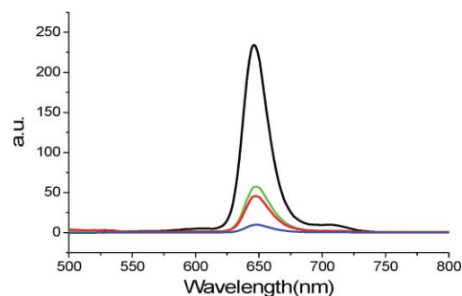
Fig. 7 Fluorescent spectra of T1 (blue), T2 (red), T3 (green) and T4 (black) in cyclohexane (1.0 \mu\text{M} , excitation wavelength = 423 nm).
