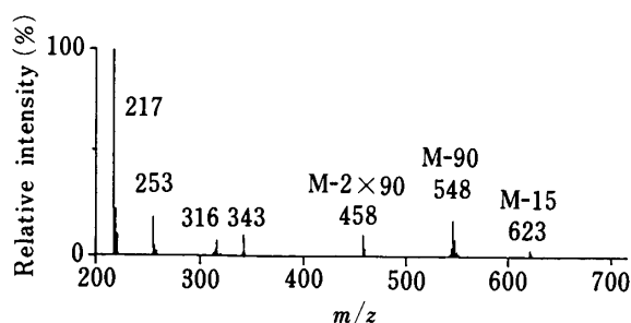
Fig. 2. Mass Spectrum of the Methyl Ester-Trimethylsilyl Ether of 1\beta,3\alpha,12\alpha -Trihydroxy- 5\beta -cholan-24-oic Acid in Urine from a Healthy Man
