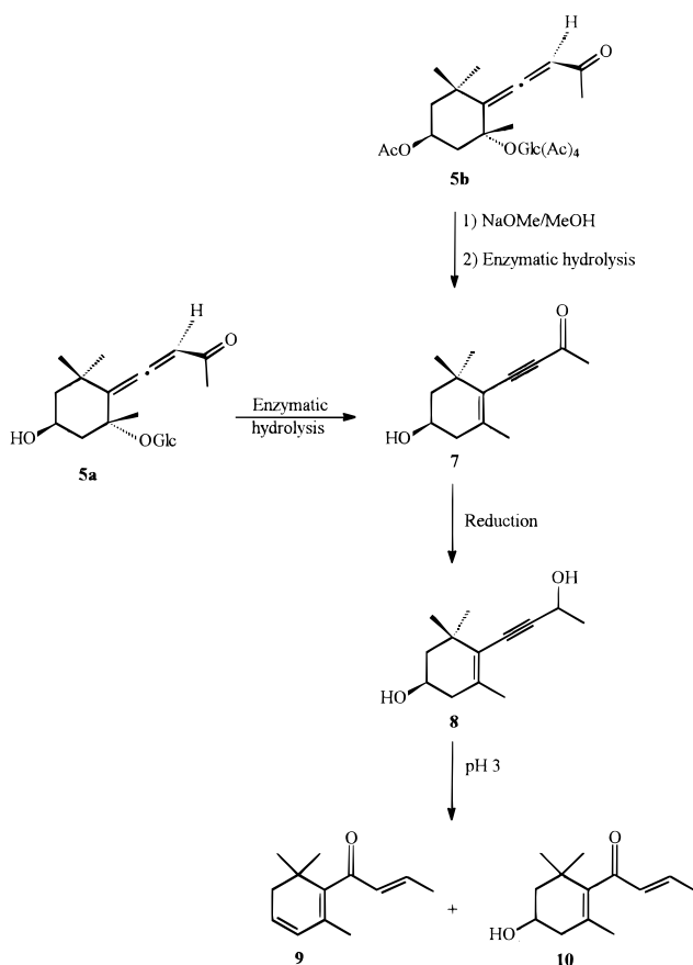
Figure 2. Generation of 3-hydroxy-7,8-didehydro- \beta -ionone ( 7 ), \beta -damascenone ( 9 ), and 3-hydroxy- \beta -damascenone ( 10 ) from (3 S ,5 R ,8 R )-3,5-dihydroxy-6,7-megastigmadien-9-one 5- O - \beta -D-glucopyranoside ( 5a ).
