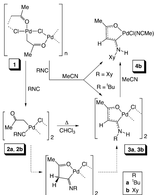
Scheme 2
