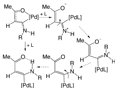
Scheme 5
