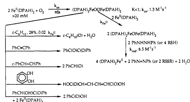
Scheme I. Activation of O 2 by Fe II (DPAH) 2 in 1.8:1 py/HOAc
