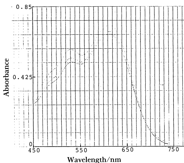
Fig. 2. Visible spectra of \text{Fe}(\text{bpy})_3^{3+} and \text{C}_6\text{H}_5\text{H}_2\text{PO}_2 at 27^\circ\text{C} in the ratio 1:0 (—), 1:1 (---), and 1:10 (-·-) where 10^4[\text{Fe}(\text{bpy})_3^{3+}] = 8.0 and [\text{H}^+] = 2.5 \text{ mol dm}^{-3} .
