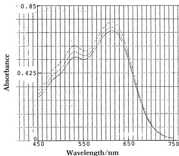
Fig. 1. Visible spectra of the mixtures of \text{Fe}(\text{bpy})_3^{3+} and \text{H}_3\text{PO}_2 at 27^\circ\text{C} in the ratio 1:0 (—), 1:1 (---), and 1:10 (-·-) where [\text{Fe}(\text{bpy})_3^{3+}] = 8.0 \times 10^{-4} \text{ mol dm}^{-3} , and [\text{H}^+] = 2.5 \text{ mol dm}^{-3} .
