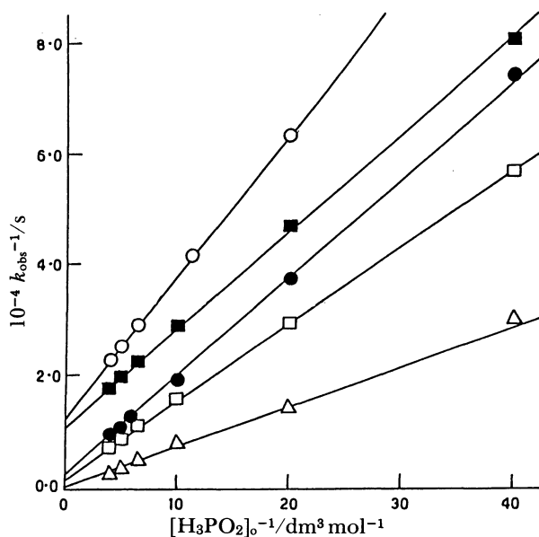
Fig. 4. Plot between k_{\text{obs}}^{-1} and [\text{H}_3\text{PO}_2]_o^{-1} at different temperatures for the oxidations affected by \text{Fe}(\text{phen})_3^{3+} at 30°C (■), 40.5°C (□), and 50°C (△) and for the oxidations by \text{Fe}(\text{bpy})_3^{3+} at 30°C (○) and 40.5°C (●).
