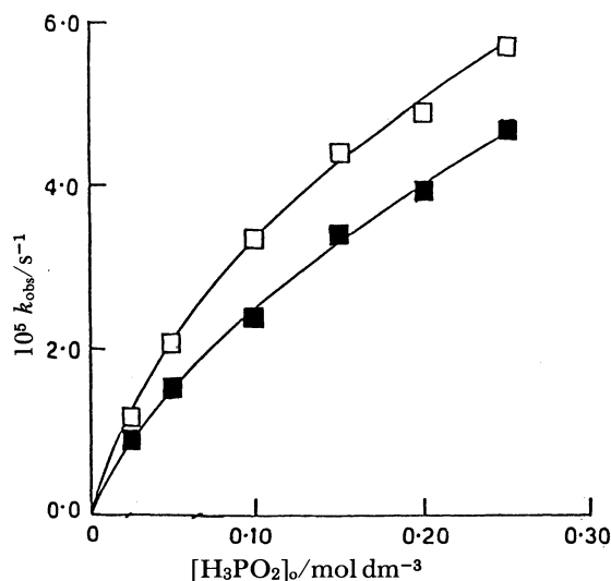
Fig. 3. Plot between k_{obs}(s^{-1}) and [H_3PO_2] at 30 °C with 10^4[Fe(phen)_3^{3+}]=0.632 and [H^+]=0.5 and I=1.0 \text{ mol dm}^{-3} (□) and with 10^4[Fe(bpy)_3^{3+}]=0.729 and [H^+]=0.5 and I=1 \text{ mol dm}^{-3} at 30 °C (■).
