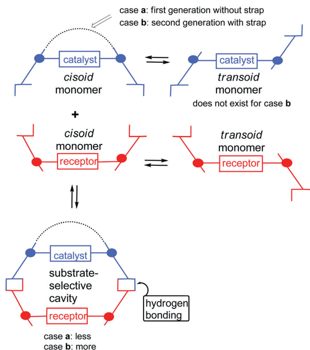
Fig. 1 The principles of our substrate-selective epoxidation catalysis. The substrate-selective catalytic cavity self-assembles from the equilibrium mixture of its monomers. First generation (a) : the catalyst part does not contain a strap. Second generation (b) : the catalyst part contains a strap forcing the catalyst part to be in a cisoid conformation, thus increasing the amount of the substrate-selective cyclic cavity and hampering non-selective catalysis on the outside of the cavity. The formation of oligomers of the catalyst part and the receptor part is omitted for clarity.
