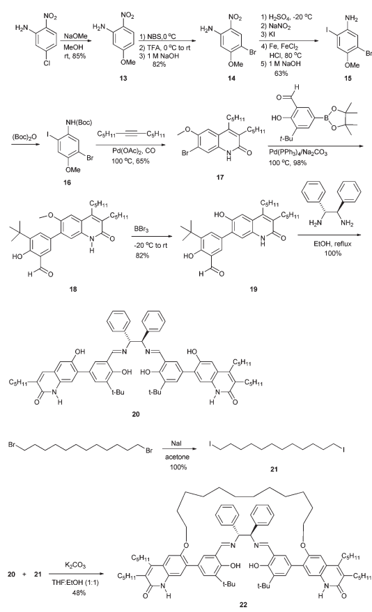
Scheme 1 Synthesis of strapped catalyst part 8 .
