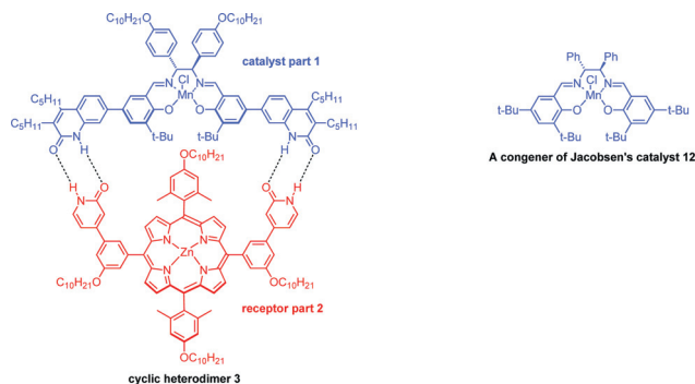
Fig. 2 The first generation of the supramolecular catalytic system (model: 1 + 2 \rightleftharpoons 3 ). A congener of Jacobsen's catalyst, 5a compound 12 .
