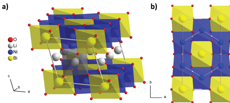
Figure 1. (a) Representation of the A_3M_2XO_6 structure in the case of Li_3Ni_2BiO_6 in perspective view, evidencing the layered organization of Ni_{2+}/Bi_{5+}O_2 slabs (blue and yellow edge-shared octahedra) and LiO_2 interslab (in gray, only one octahedron is drawn for clarity). (b) Representation along the monoclinic c axis highlighting the honeycomb-type Ni^{2+}/Bi^{5+} ordering within the slab.
