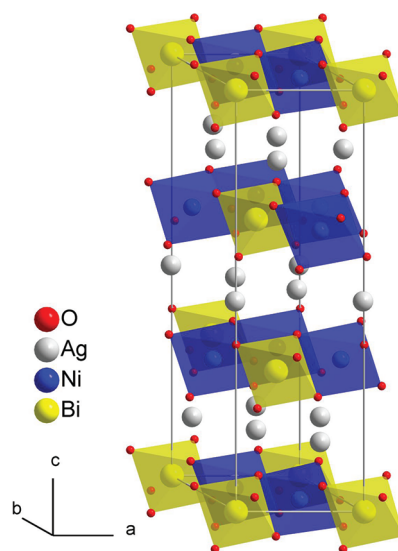
Figure 10. Representation in a perspective view of the Ag 3 Ni 2 BiO 6 delafossite structure. The honeycomb Ni 2+ /Bi 5+ ordering is evidenced within the Ni 2/3 Bi 1/3 O 2 slabs (blue and yellow edge-shared octahedra), while Ag cations (in gray) occupy dumbbell linear sites.
