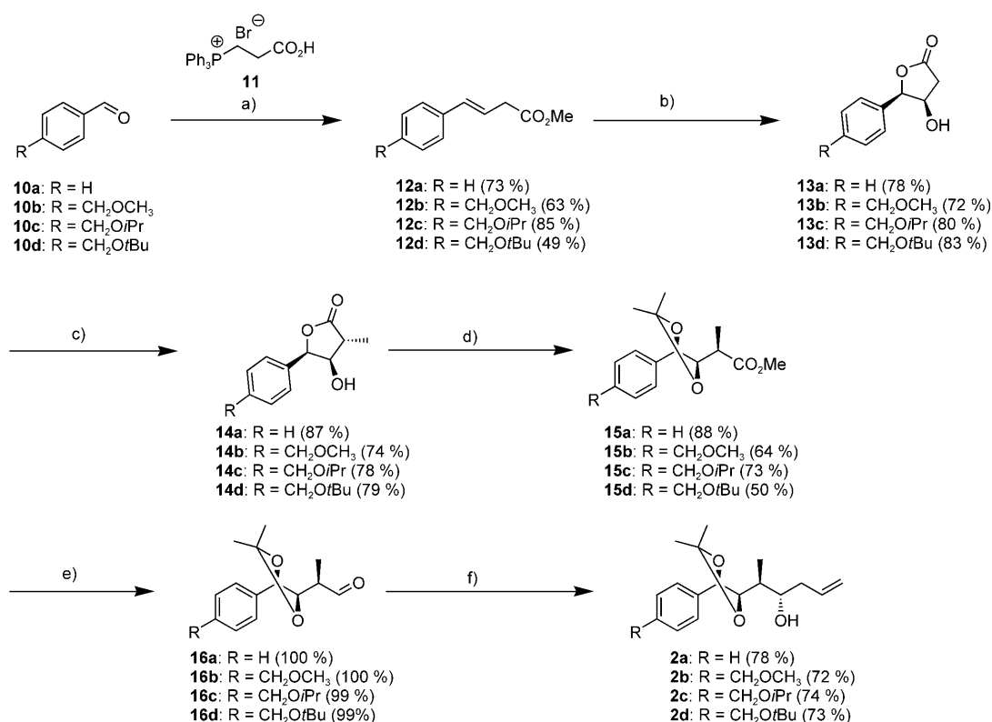
Scheme 3. Synthesis of unit A building blocks. a) t BuOK, THF, -50^\circ\text{C} to RT, then MeI; b) \text{K}_2\text{OsO}_4 \cdot 2\text{H}_2\text{O} , (DHQD) 2 -PHAL, \text{K}_3[\text{Fe}(\text{CN})_6] , \text{K}_2\text{CO}_3 , \text{H}_2\text{O}/i\text{BuOH} , 0^\circ\text{C} ; c) LDA, MeI, THF, -100^\circ\text{C} to -78^\circ\text{C} ; d) \text{Me}_2\text{C}(\text{OMe})_2 , MeOH, Amberlyst-15, at RT; e) DIBAL-H, \text{CH}_2\text{Cl}_2 , -78^\circ\text{C} ; f) \text{CH}_2=\text{CHCH}_2\text{Sn}(\text{nBu})_3 , \text{MgBr}_2 \cdot \text{Et}_2\text{O} , \text{CH}_2\text{Cl}_2 , -78^\circ\text{C} .
