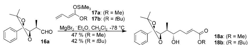
Scheme 5. Vinyllogous Mukaiyama aldol addition mediated by \text{MgBr}_2 \cdot \text{Et}_2\text{O} .
