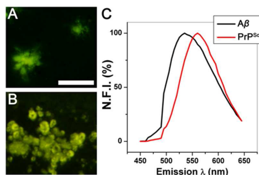
Figure 1. True color imaging of amyloid deposits in tissue stained with ANCA probe 1. (A) A \beta deposits in the hippocampus of an AD mouse model. (B) PrP Sc deposits in the corpus callosum of a prion-infected mouse. (C) Ex vivo fluorescence spectra of stained deposits showing distinct emission maxima for A \beta and PrP Sc . Scale bar = 100 \mu m. NFI = normalized fluorescence intensity.
