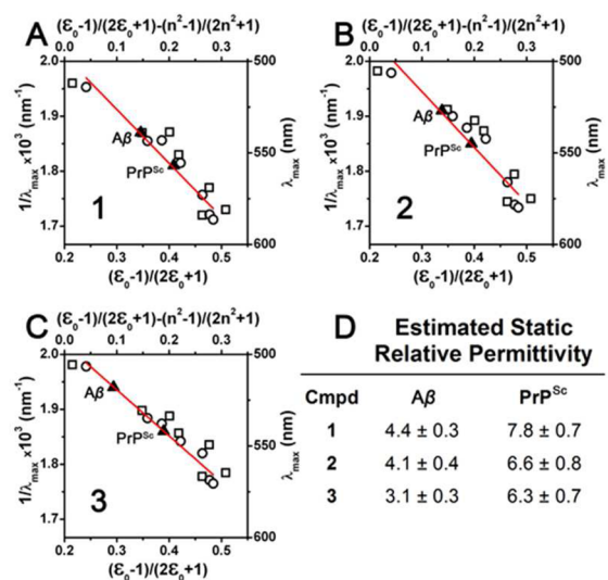
Figure 2. Dependence of fluorescence emission of probes 1 – 3 on the polarity of different organic solvents. (A–C) Graphs of the relationship between 1/\lambda_{\text{max}} for emission of 1 – 3 as functions of solvent static relative permittivity ( \epsilon_0 ), with ( \square ) or without ( \circ ) the contribution of refractive index ( n ). For each graph, the linear fits of the data according to eq 2 are shown in red, excluding the contribution from n . (D) Estimated \epsilon_0 for the binding pockets of A \beta and PrP Sc deposits extrapolated from the observed \lambda_{\text{max}} for emission of 1 – 3 in tissue samples.
