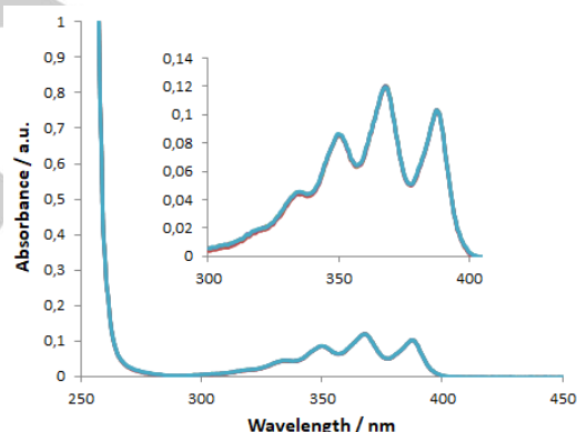
Figure 3 Time course spectra of [Ag(EIA)_2]Cl ( 10^{-5} M, phosphate buffer 50 mM pH 7.4, 1% DMSO) for 24 h; see supporting material for UV-Vis spectrum in pure DMSO and DMF.
