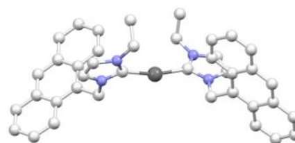
Figure 2 X-ray structure of complex [Ag(EIA)_2]Cl : C-Ag bond length 2.093(4) Å and c-Ag-C' angle 167.7^\circ (C' is reported by the symmetry operation -x+1, +y, -z-1/2 ).
