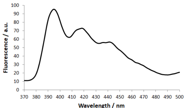
Figure 4 Emission spectra of [Ag(EIA) 2 ]Cl ( 10^{-6} M in 50 mM phosphate buffer pH 7.4 in presence of 0.001% DMSO) \lambda_{exc}=350 nm.
