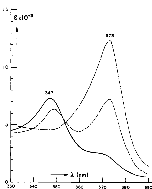
Figure 1. (—) Optical spectrum of difluorenylbarium in tetrahydrofuran at 25°; (---) 1:1 complex of 4'-methylbenzo-18-crown-6 and \text{Ba}^{2+}, \text{Fl}_2^{2-} ( \text{Fl}^- , \text{Ba}^{2+} , crown, \text{Fl}^- ); (-·-) 2:1 complex of 4'-methylbenzo-15-crown-5 and \text{Ba}^{2+}, \text{Fl}_2^{2-} ( \text{Fl}^- , crown, \text{Ba}^{2+} , crown, \text{Fl}^- ).
