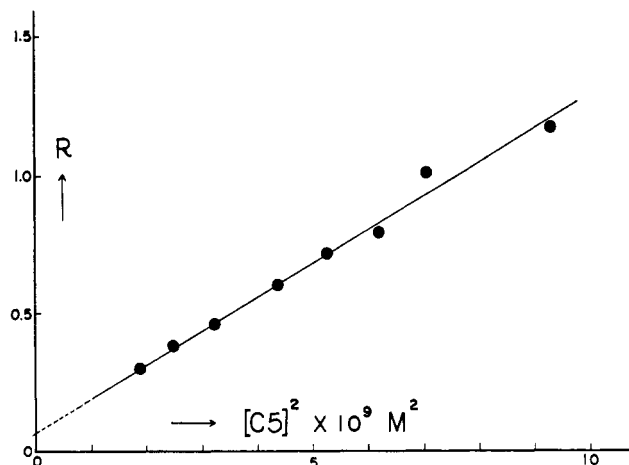
Figure 4. Plot of ratio R ( = [\text{loose ion pairs}]/[\text{tight ion pairs}] ) vs. square of crown concentration for the system difluorenylbarium and 4'-methylbenzo-15-crown-5 in THF at 25°.
