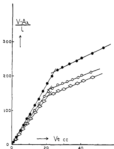
Figure 2. Titration plots V \cdot A_\lambda / l vs. V_t for difluorenylbarium in THF at 25° with (●) 4'-methylbenzo-18-crown-6, (○) glyme-9 (octaethylene glycol dimethyl ether), and (◊) glyme-7 (hexaethylene glycol dimethyl ether).
