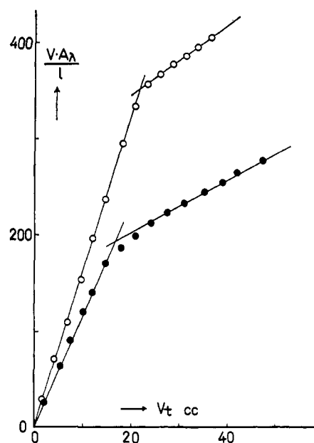
Figure 3. Titration plots V \cdot A_\lambda / l vs. V_t for difluorenylbarium in THF at 25° with (○) poly(vinylbenzo-15-crown-5) and (●) poly(vinylbenzo-18-crown-6).
