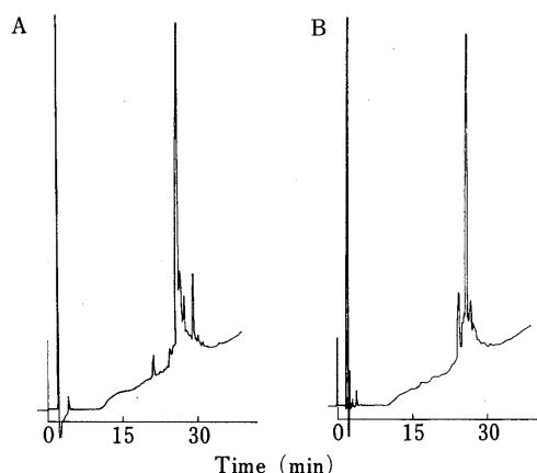
Fig. 3. Analytical HPLC of Crude Human Pancreastatin-29
