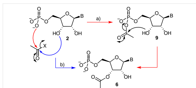
Scheme 1 Potential pathways for nucleotide acetylation: a) intramolecular acyl transfer from mixed anhydride 9 ; b) direct hydroxyl acylation; B = nucleobase; X = nucleofuge.
