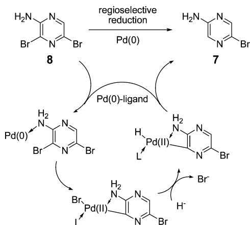
Scheme 3. Mechanism of the regioselective debromination
