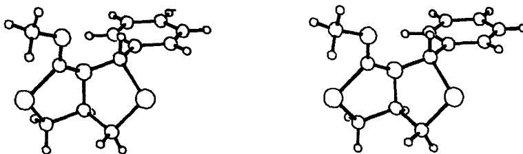
Fig. 4. Stereoscopic drawing of 9d
