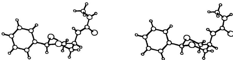
Fig. 1. Stereoscopic drawing of 7d
