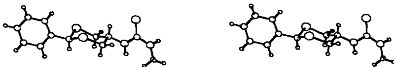
Fig. 2. Stereoscopic drawing of 8d
