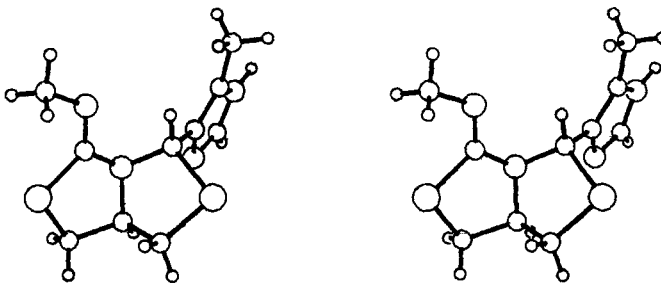
Fig. 3. Stereoscopic drawing of 9a
