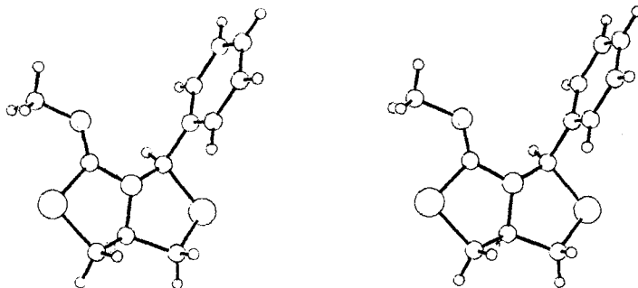
Fig. 5. Stereoscopic drawing of 10d
