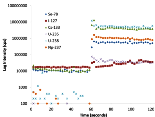
Figure 2. Typical LA-ICP-MS spectrum for \text{CsUSeO}+\text{Np}^{\text{VI}} showing the initial 60 s background with the laser shutter in place followed by the 60 s ablation measurement. The relatively flat profile of the ablation data indicates that the constituent elements are present uniformly in the crystal.
