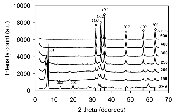
Figure 4. XRD analysis of residual products collected at various times during thermal combustion of ZHA in air (50–600 °C). Samples were heated at 20 °C/min to the final temperature shown on the right. ZnO expected peak positions are shown with sticks on the bottom of the figure; Miller indices are labeled on the top.
