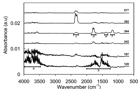
Figure 7. FTIR spectra of evolved gaseous products collected at the temperature (°C) indicated on the right of each spectrum during thermal combustion of ZNA in air (20 °C/min). FTIR spectra were scaled by dividing by 10 except for those at 120 and 197 °C which were not scaled. Expected positions of absorption bands for water stretching modes (a), bending mode (b), CO 2 antisymmetric stretch (c), overlapping acetic acid and acetone C=O stretch (d), CH 3 deformation (e), and C–C bending for acetone and C–O stretch for acetic acid (f) are shown.
