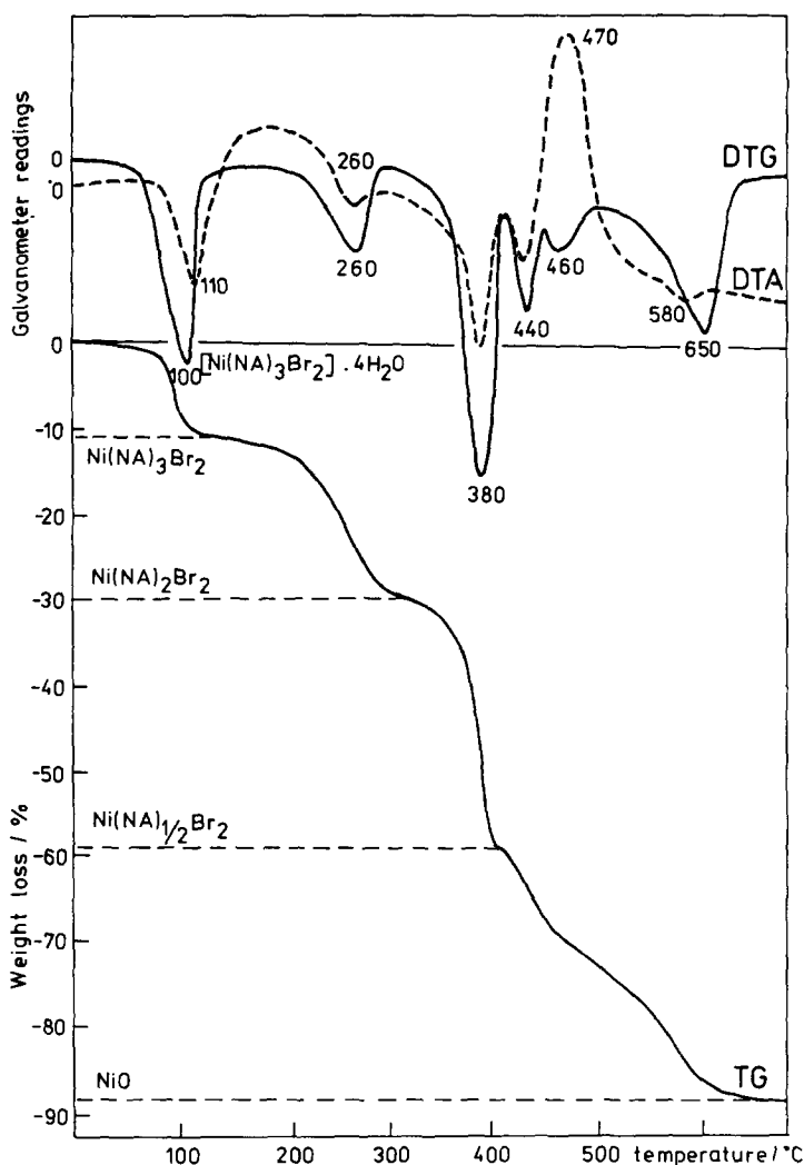
Fig. 2. Thermal curves of \text{Ni(NA)}_3\text{Br}_2 \cdot 4\text{H}_2\text{O} .
