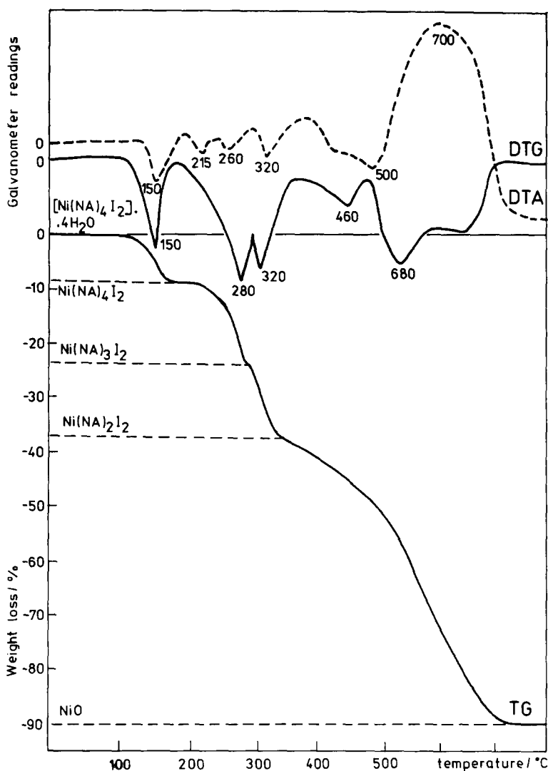
Fig. 3. Thermal curves of \text{Ni(NA)}_4\text{I}_2 \cdot 4\text{H}_2\text{O} .
