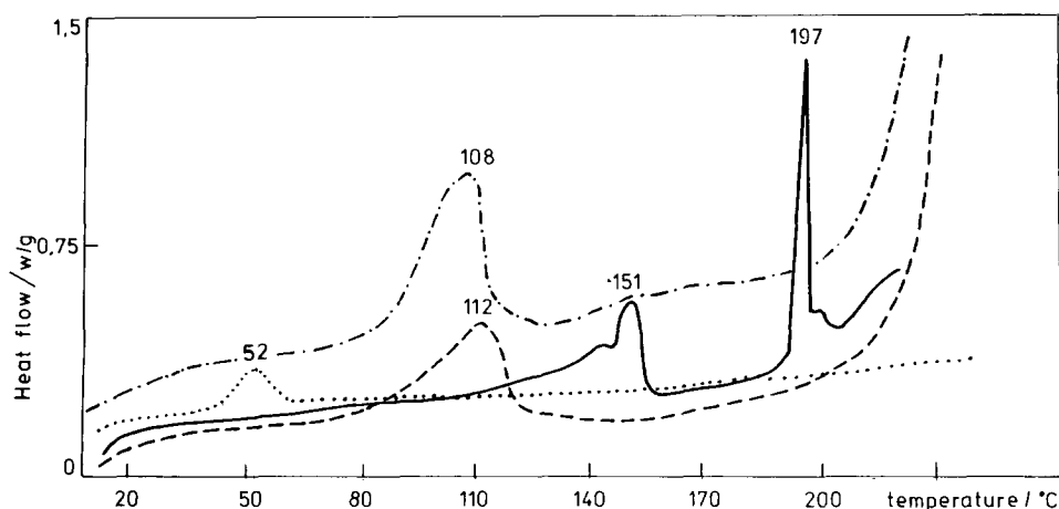
Fig. 6. DSC curves of [\text{Ni}(\text{NA})_n\text{X}_2] \cdot n\text{G} complexes: \cdots , X is Cl, n\text{G} = 2\text{H}_2\text{O} ; -\cdots- , X is Br, n\text{G} = 2\text{H}_2\text{O} ; ---- , X is I, n\text{G} = 4\text{H}_2\text{O} ; ———— , X is NCS, n\text{G} = 2\text{C}_2\text{H}_5\text{OH} .
