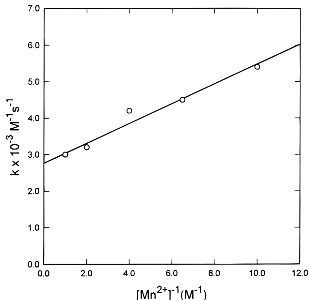
Figure 7. Rate constant of the \text{Mn}^{3+} + \text{H}_2\text{O}_2 reaction as a function of the reciprocal \text{Mn}^{2+} concentration (1 krad, 22 °C, in 1.0 M \text{HClO}_4 ).
