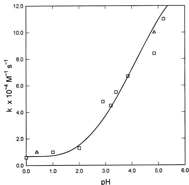
Figure 8. Apparent rate constant of \text{Mn}^{3+} + \text{H}_2\text{O}_2 as a function of pH in ( \square ) \text{HClO}_4 and ( \Delta ) \text{H}_2\text{SO}_4 solutions (1 krad, 22 °C, with [\text{Mn}^{2+}] = 0.1 \text{ M} ).
