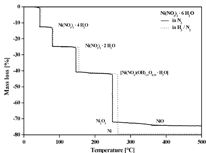
Fig. 3. Thermal decomposition (TG) of nickel(II)nitrate hexahydrate in inert/ N_2 atmosphere (full line) and in reducing/ H_2/N_2 (10% H_2 ) atmosphere (dotted/broken line) with indicated degradation steps/stages. Heating rate between the quasi-isothermal steps: 0.6\text{ K min}^{-1} .
