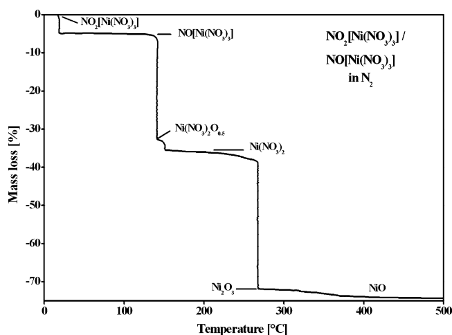
Fig. 4. Thermal decomposition (TG) of nitryl/nitrosyl nitrate nickelate in N_2 atmosphere up to 500^\circ\text{C} with indicated degradation steps/stages. Sample loading: 120 mg; heating rate between the quasi-isothermal steps: 0.6\text{ K min}^{-1} .
