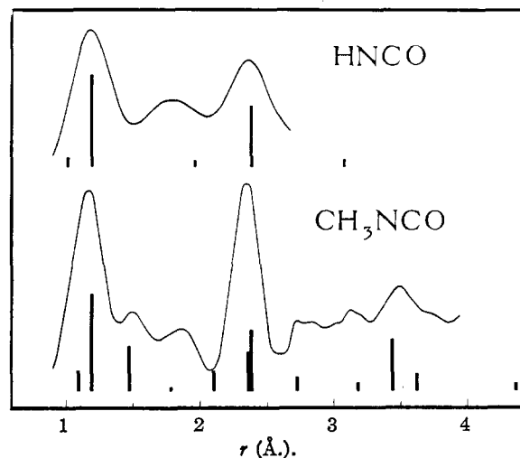
Fig. 1.—Radial distribution functions for methyl isocyanate and cyanic acid. The heavy lines correspond to the distances in the final models, and their heights are proportional to the appropriate products Z_i Z_j .
