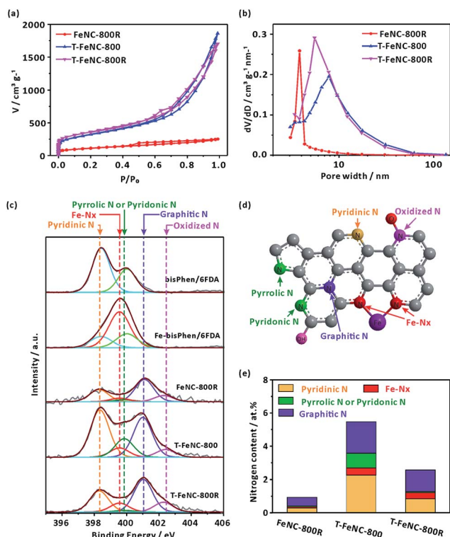
Fig. 2 (a) N 2 adsorption-desorption isotherms and (b) the pore size distribution of catalysts. (c) N 1s XPS spectra of different samples. (d) Schematic illustration of different nitrogen species. (e) Content of different N species in FeNC-800R, T-FeNC-800 and T-FeNC-800R.
