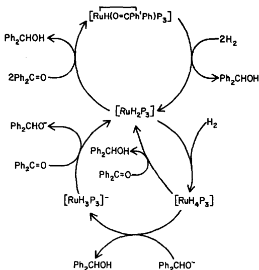
Fig. 1. Catalytic cycles for the [\text{RuH}_4\text{P}_3] -, [\text{RuH}_2\text{P}_3] - and [\text{RuH}_3\text{P}_3]^- -catalyzed hydrogenation of benzophenone ( \text{P} = \text{PPh}_3 ).
