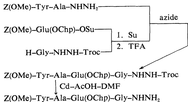
Fig. 8. Synthetic Scheme for the Protected Tetrapeptide Hydrazide, Z(OMe)-(hGIP 1—4)-NHNH 2 [8]
