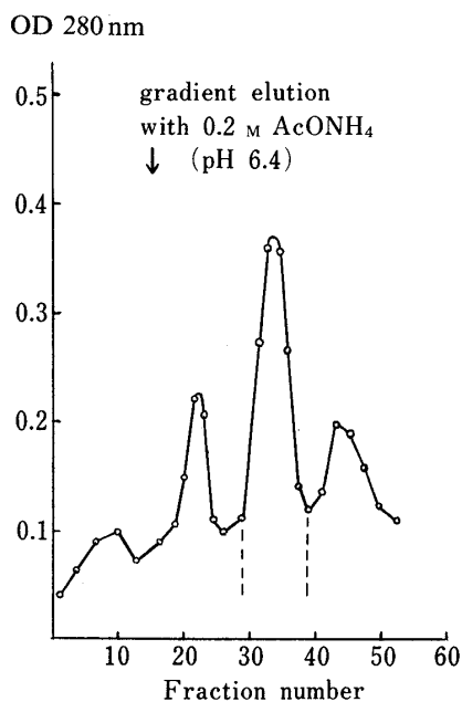
Fig. 10. CM-Cellulose Purification of Synthetic hGIP
