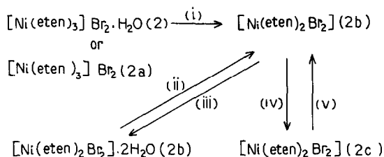
Scheme 2. (i) 220 °C; (ii) 80–142 °C; (iii) ca. 3 h in humid atmosphere (relative humidity 60–70%) at ambient temperature; (iv) 50–76 °C; \Delta H = 1.2 \text{ kJ mol}^{-1} ; (v) 49–85 °C; \Delta H = -0.8 \text{ kJ mol}^{-1} .
