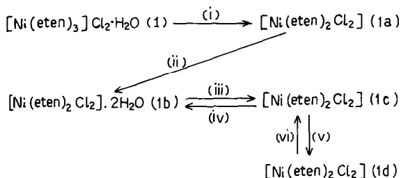
Scheme 1. (i) 68–166 °C; (ii) crystallization from aqueous methanol or ethanol; (iii) 70–98 °C; (iv) ca. 3 h in humid atmosphere (relative humidity 60–70%) at ambient temperature; (v) 182–200 °C; \Delta H = 2.9 \text{ kJ mol}^{-1} ; (vi) complete reversion takes place in ca. 30 min.
