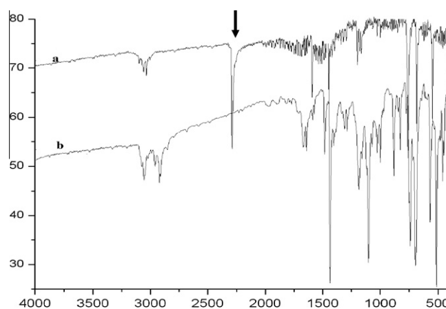
Fig. 1. IR spectra of: (a) PdCl 2 (PhCN) 2 before addition of dpme ligand and (b) after the addition to prepare 1 .
