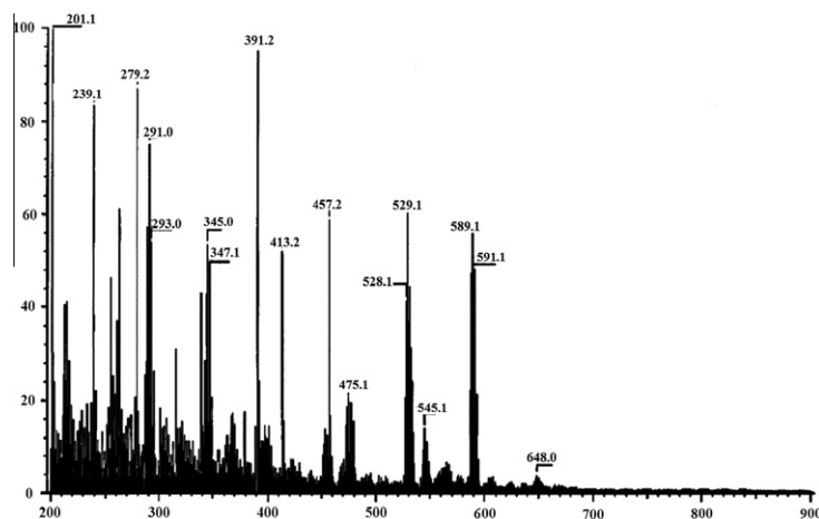
Fig. 2. FAB-MS Spectrum of 2.
