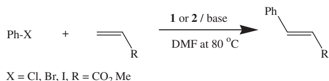
Scheme 2. The Heck coupling reaction of benzene halide with methyl acrylate to prepare cinnamate.
