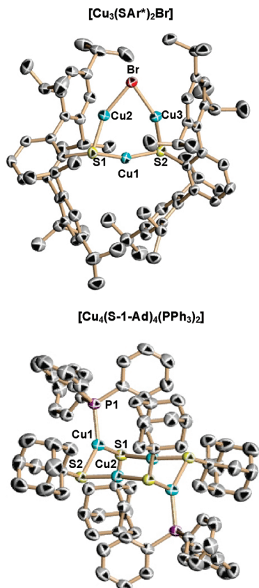
Figure 3. Structures of polynuclear Cu I complexes showing 50% probability ellipsoids, partial atom numbering schemes, and selected bond distances (Å) and angles (deg). [Cu 3 (Ar * S) 2 Br] (upper): Cu1–S1 2.174(1), Cu1–S2 2.173(1), Cu2–S1 2.186(1), Cu3–S2 2.198(1), Cu2–Br 2.301(1), Cu3–Br 2.317(1), S1–Cu1–S2 161.27(3), Cu1–S1–Cu2 77.59(2), Cu1–S2–Cu3 73.36(2), S1–Cu2–Br 149.43(2), S2–Cu3–Br 148.24(2), Cu2–Br–Cu3 74.40(1). [Cu 4 (S-1-Ad) 4 (PPh 3 ) 2 ] (lower, crystallographically imposed centrosymmetry): Cu1–P1 2.252(1), Cu1–S1 2.286(1), Cu1–S2 2.227(1), Cu2–S2 2.173(1), Cu2–S1 2.157(1), P1–Cu1–S1 105.75(3), P1–Cu1–S2 139.47(3), S1–Cu1–S2 113.34(3), S2–Cu2–S1' 165.71(3).
