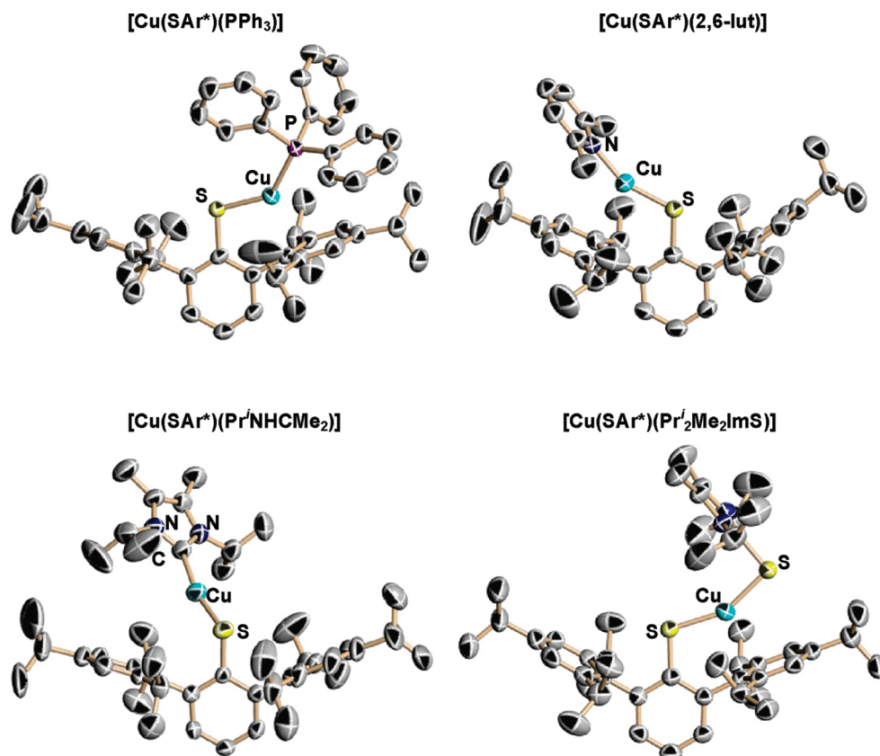
Figure 4. Structures of quasi-two-coordinate \text{Cu}^{\text{I}} complexes [\text{Cu}(\text{SAr}^*)\text{L}] : \text{L} = \text{PPh}_3 and 2,6-lut (upper) and \text{Pr}^i_2\text{NHCMe}_2 and \text{Pr}^i_2\text{Me}_2\text{ImS} (lower), showing 50% probability ellipsoids. Metric data are summarized in Table 2.
