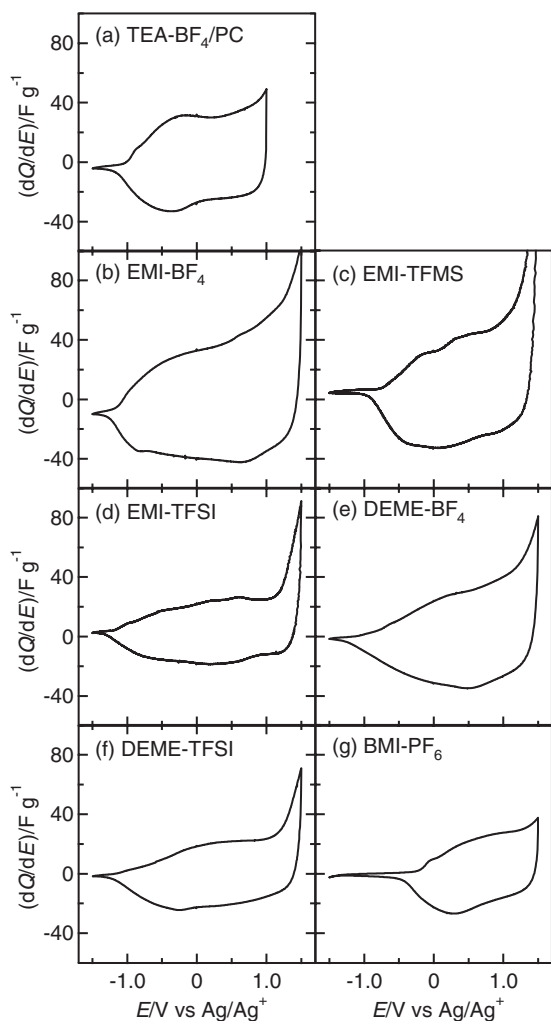
Figure 1. Cyclic voltammograms of NiO/Ni in various electrolytes at 2 mV s -1 .
