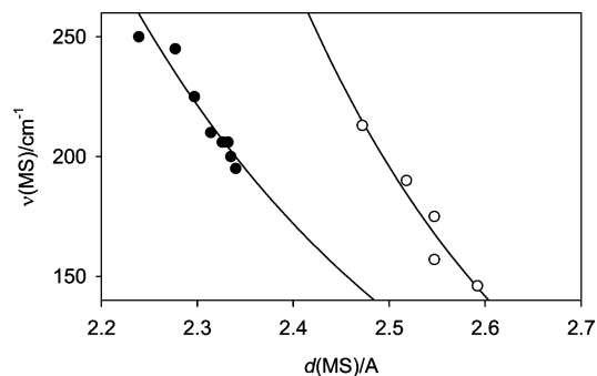
Figure 7. Correlation between \nu(\text{MS}) and the M–S bond length d(\text{MS}) for \text{AgNO}_3/\text{tu} (1:3), 1 , and \text{AgNO}_3/\text{tu} (15:23), 3 (○) (M = Ag; this work), and for \text{Cu}_2\text{SO}_4/\text{tu}/\text{H}_2\text{O} (1:5:3) and \text{Cu}_2\text{SO}_4/\text{tu}/\text{H}_2\text{O} (1:6:1) (●) (M = Cu; data from ref 11).
