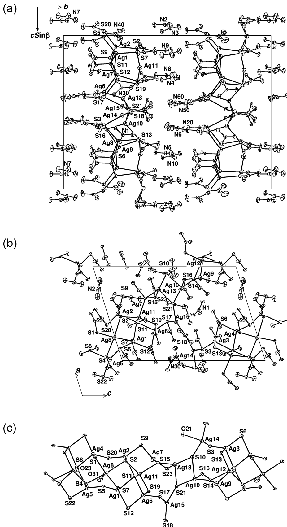
Figure 4. (a) Unit cell contents of \text{AgNO}_3/\text{tu} (15:23), 3 , down a , showing the partitioning of the cell contents at y = 0, 0.5 . (b) Projections of the unit cell contents down b , showing cross-linking of the polymer strands by \text{tu}(18) . (c) A single strand of the cation polymer, showing the \text{Ag,S(O)} framework only. Within the \text{Ag/S} framework, the following rings are identified ( \text{Ag,S} by number, S italicized, primed atoms related by the unit c translation): (a) four-membered rings, a_1 3, 4', 6, 8'; a_2 7, 13, 15, 23; a_3 1, 6, 11, 12; a_4 10, 13, 10, 21; a_5 9, 10, 14, 16; (b) six-membered rings, b_1 5', 9, 12, 4', 14, 22'; b_2 3, 5', 12, 4', 13, 8'; b_3 1, 5, 8, 4, 5, 7; b_4 2, 7, 11, 2, 9, 15; b_5 2, 6, 11, 2, 11, 19; (c) eight-membered rings, c_1 1, 4, 5, 8, 1, 5, 7, 8; c_2 1, 2, 4, 8, 1, 7, 11, 20; c_3 6, 11, 13, 15, 15, 17, 19, 21; c_4 3, 10, 12, 14, 3, 10, 13, 14.
