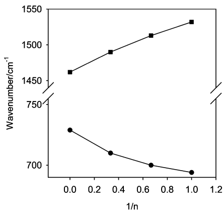
Figure 5. Plot of the \nu(\text{CS}) and \nu_a(\text{CN}) wavenumbers for \text{AgNO}_3/\text{tu} (1: n ) ( n = 1, 1.5 , and 3 ; 4 , 2 , and 1 ) and uncomplexed \text{tu} ( n = \infty ) as a function of 1/n .
