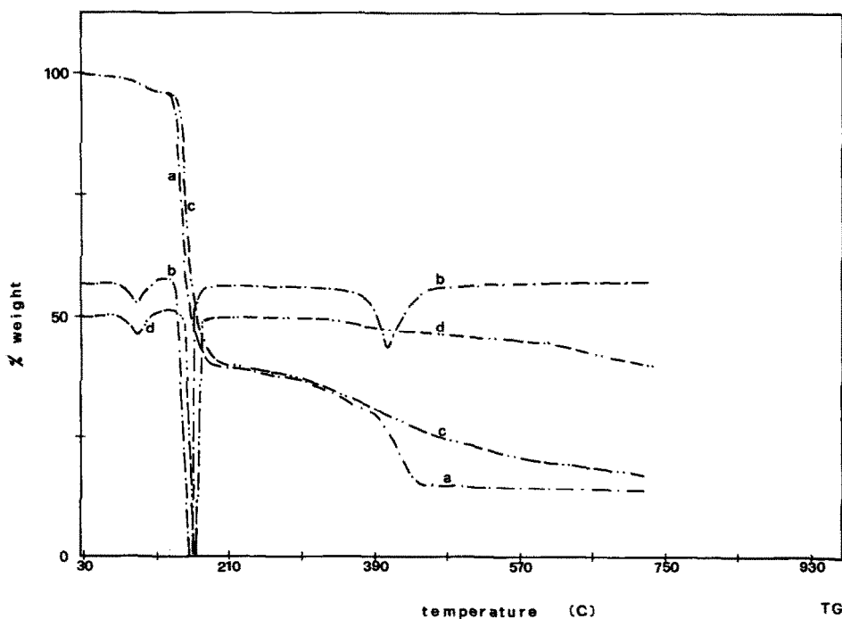
Fig. 4. TG and DTG curves of \text{Cu}(\text{2mIm})_4(\text{NO}_3)_2 : a and b, air atmosphere; c and d, nitrogen atmosphere. Heating rate 10^\circ\text{C min}^{-1} .
