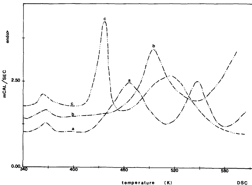
Fig. 3. DSC curves of: a, \text{Co}(\text{2mIm})_4(\text{NO}_3)_2 ; b, \text{Ni}(\text{2mIm})_4(\text{NO}_3)_2 ; c, \text{Cu}(\text{2mIm})_4(\text{NO}_3)_2 . Nitrogen atmosphere; heating rate 10^\circ\text{C min}^{-1} .
