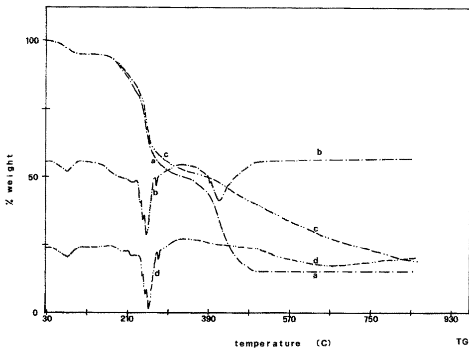
Fig. 1. TG and DTG curves of \text{Co}(\text{2mIm})_4(\text{NO}_3)_2 , form A: a and b, air atmosphere; c and d, nitrogen atmosphere. Heating rate 10^\circ\text{C min}^{-1} .
