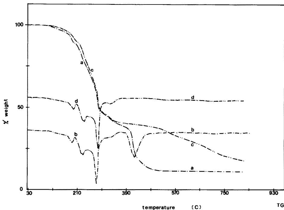
Fig. 8. TG and DTG curves of \text{Ni}(\text{4mIm})_6(\text{NO}_3)_2 : a and b, air atmosphere; c and d, nitrogen atmosphere. Heating rate 10^\circ\text{C min}^{-1} .
