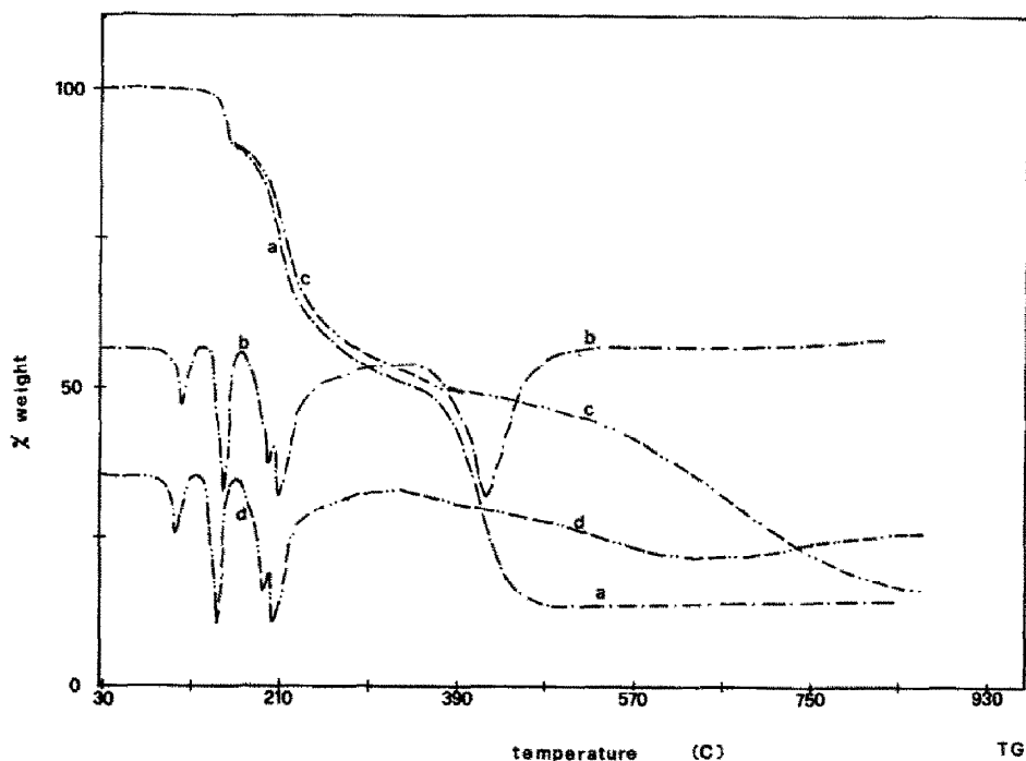
Fig. 5. TG and DTG curves of \text{Co}(\text{2mIm})_4(\text{NO}_3)_2 , form B: a and b, air atmosphere; c and d, nitrogen atmosphere. Heating rate 10^\circ \text{C min}^{-1} .
