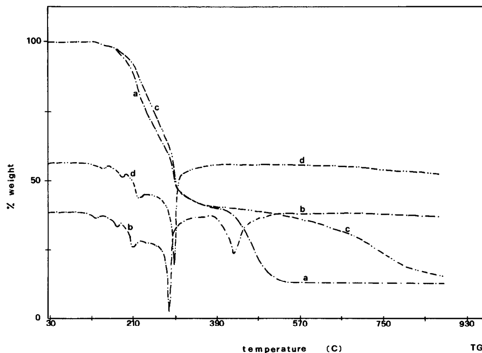
Fig. 7. TG and DTG curves of \text{Co}(\text{4mIm})_6(\text{NO}_3)_2 : a and b, air atmosphere; c and d, nitrogen atmosphere. Heating rate 10^\circ\text{C min}^{-1} .
