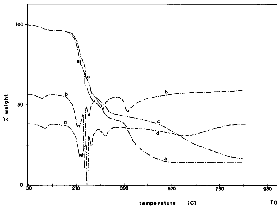
Fig. 6. TG and DTG curves of \text{Ni}(\text{2mIm})_4(\text{NO}_3)_2 , form B: a and b, air atmosphere; c and d, nitrogen atmosphere. Heating rate 10^\circ\text{C min}^{-1} .
