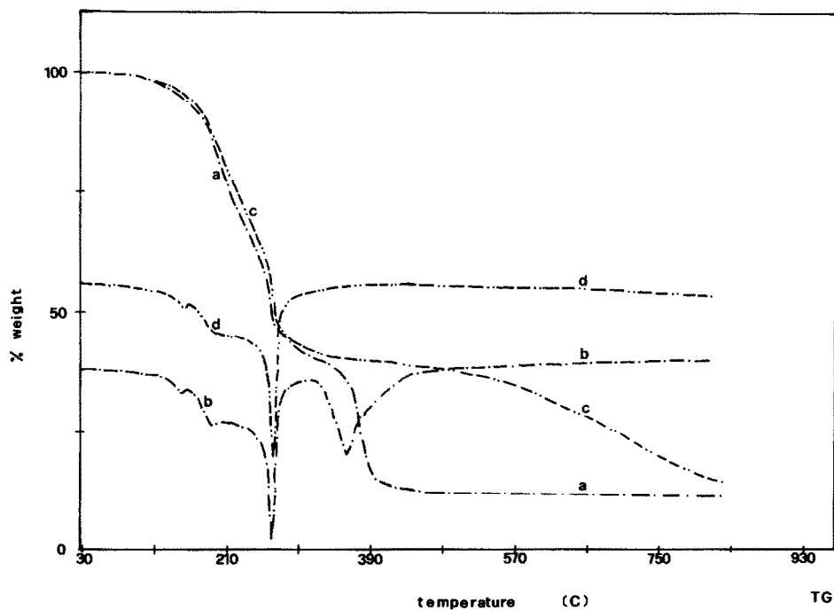
Fig. 9. TG and DTG curves of \text{Cu}(\text{4mIm})_6(\text{NO}_3)_2 : a and b, air atmosphere; c and d, nitrogen atmosphere. Heating rate 10^\circ\text{C min}^{-1} .
