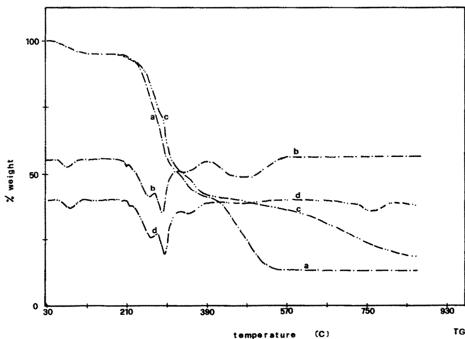
Fig. 2. TG and DTG curves of \text{Ni}(\text{2mIm})_4(\text{NO}_3)_2 , form A: a and b, air atmosphere; c and d, nitrogen atmosphere. Heating rate 10^\circ\text{C min}^{-1} .
