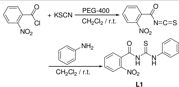
Scheme-I: Synthetic route of L1
