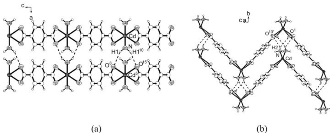
Fig. 5 Hydrogen bonding between the [\text{Cd}(\mu\text{-bdc})(\text{NH}_3)_2] -chains in 2 (a) along a and (b) along b ; see Table 1 for details, symmetry operations: ^1 = x, y+1, z ; ^5 = x+1/2, y+1/2, z ; ^8 = -x+1/2, y+1/2, -z+1/2 ; ^{10} = x, y, -z+1/2 ; ^{10'} = x, y+1, -z+1/2 ; ^{15} = -x+1/2, y+1/2, z .
