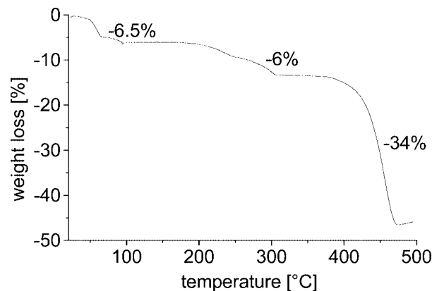
Fig. 6 TGA curve of [\text{Cd}(\mu\text{-bdc})(\text{NH}_3)_2] ( 2 ).
