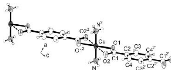
Fig. 1 Straight-chain structure of \frac{1}{\infty}[\text{Cu}(\mu\text{-bdc})(\text{NH}_3)_2] in 1.
