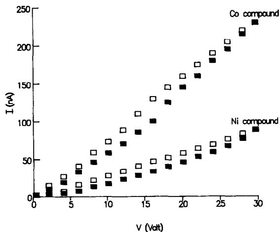
Fig. 4. Room temperature plot of current ( I ) versus voltage ( V ) for discs of \text{Co}(\text{C}_{13}\text{H}_9\text{N})\text{Cl}_2 and \text{Ni}(\text{C}_{13}\text{H}_9\text{N})\text{Cl}_2 : ■, V increasing; □, V decreasing.
