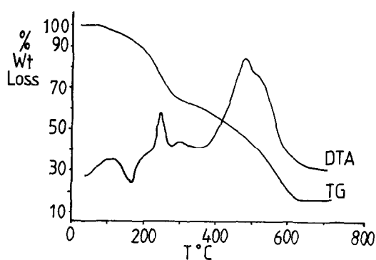
Fig. 3. TG and DTA trace for \text{Cu}(\text{C}_{13}\text{H}_9\text{N})_2\text{Cl}_2 . Sample weight = 9.36 mg.
