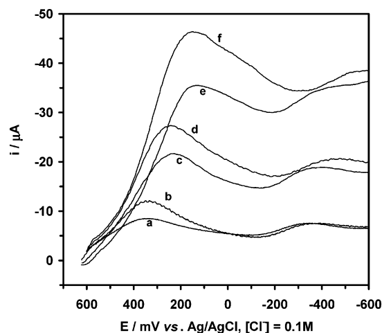
Figure 4. Reduction waves of peroxynitrous acid at pH 3.2 and 5.6 and several scan rates: 1 mM peroxynitrous acid, 0.1 M phosphoric acid/phosphate buffers; (a) pH 5.6, 1 V s -1 ; (b) pH 3.2, 1 V s -1 ; (c) pH 5.6, 4 V s -1 ; (d) pH 3.2, 4 V s -1 ; (e) pH 5.6, 10 V s -1 ; (f) pH 3.2, 10 V s -1 .
