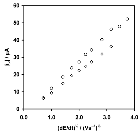
Figure 3. Peak currents vs square root of the scan rate: 1 mM peroxynitrite with 0.1 M phosphoric acid/phosphate buffers, gold electrode; circles, pH 3.2; diamonds, pH 5.6.
