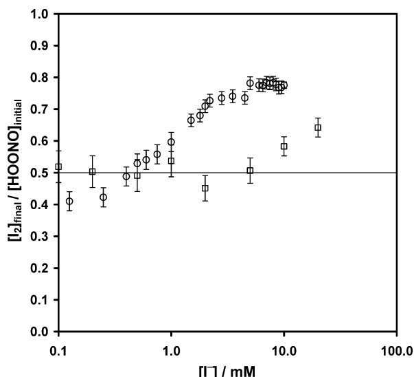
Figure 5. Relative yields of diiodine from the oxidation of iodide by peroxyntous acid vs total iodide concentration: 0.1 M phosphoric acid/phosphate buffers.; circles, [\text{HOONO}]_{\text{initial}} = 25 \mu\text{M} ; squares, [\text{HOONO}]_{\text{initial}} = 5 \mu\text{M} .
