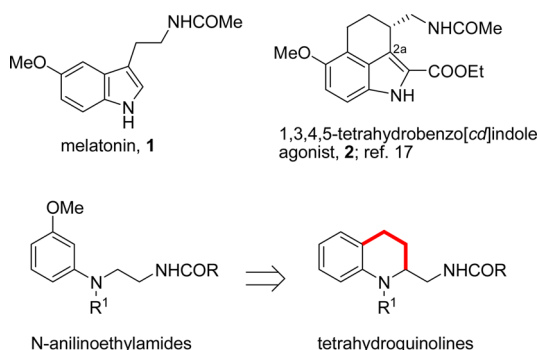
Figure 1. Structures of melatonin ( 1 ) and tetrahydrobenzo[ cd ]indole agonist 2 ; general formulas of N -anilinoethylamides and of conformationally constrained tetrahydroquinoline compounds.
