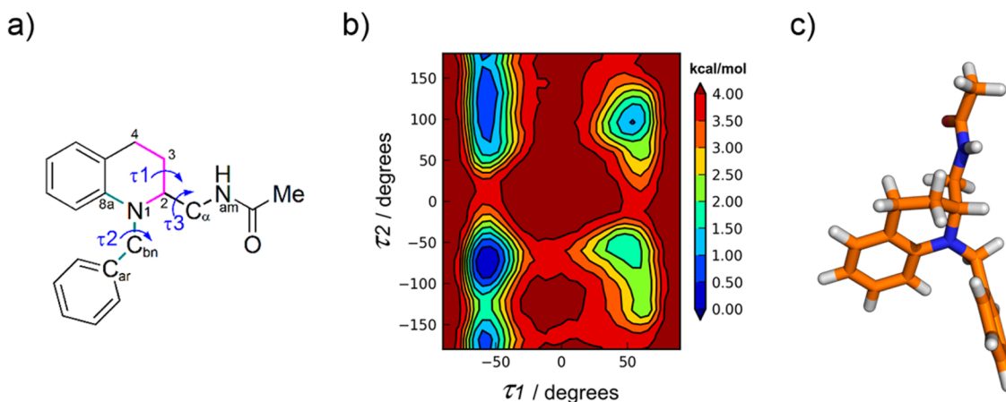
Figure 3. (a) Representation of \tau_1 ( N_1-C_2-C_3-C_4 , pink bonds), \tau_2 ( C_{8a}-N_1-C_{bn}-C_{ar} , green bonds) and \tau_3 ( N_1-C_2-C_\alpha-N_{am} ) dihedral angles. (b) Free energy surface for compound 8e obtained after 20 ns of well-tempered metadynamics simulation. (c) Representation of one of the conformations of compound 8e corresponding to the free-energy minimum ( \tau_1 = -57.7^\circ , \tau_2 = -71.1^\circ ).
