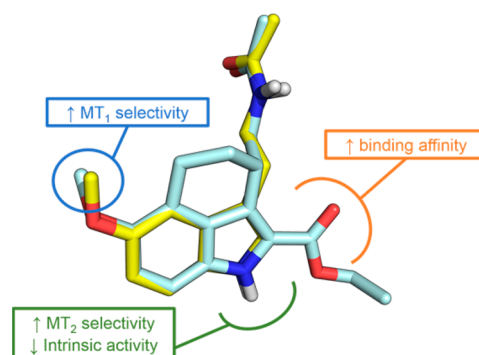
Figure 2. Superposition of compound 2 (light blue carbons) to the putative bioactive conformation of melatonin ( 1 , yellow carbons) and effect of substituents on MT 1 and MT 2 binding affinity and intrinsic activity.
