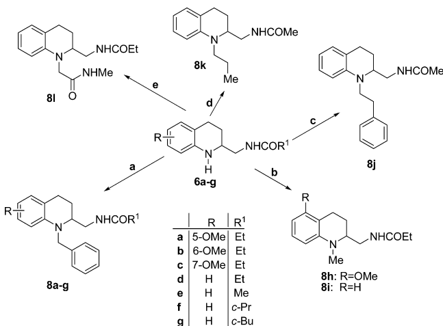
Scheme 2 a
