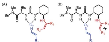
Figure 1. Proposed intermediates in Michael reactions catalyzed by 1 . (A) Favored Z-enamine. (B) Disfavored E-enamine.
