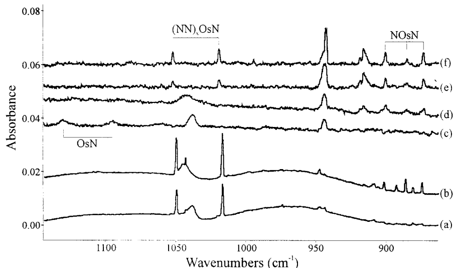
Figure 1. Infrared spectra in the 1140–860 \text{cm}^{-1} region for laser-ablated osmium atoms co-deposited with nitrogen: (a) after 1 h deposition with pure ^{14}\text{N}_2 + ^{15}\text{N}_2 (43% + 57% mixture), (b) after annealing to 25 K with pure ^{14}\text{N}_2 + ^{15}\text{N}_2 (43% + 57% mixture), (c) after 1 h deposition with 2% ^{14}\text{N}_2 + 2\% ^{15}\text{N}_2 in argon, (d) after annealing to 25 K, (e) after annealing to 40 K, (f) after annealing to 45 K. The 943 \text{cm}^{-1} band that grows on annealing is probably due to (\text{N}_2)_x\text{OsO}_2 .
