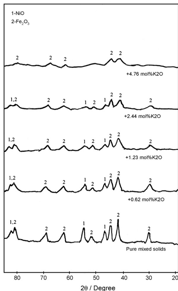
Fig. 2. X-ray diffractograms of pure mixed solids and that doped with different amounts of K 2 O followed by calcination at 300^\circ\text{C} .
