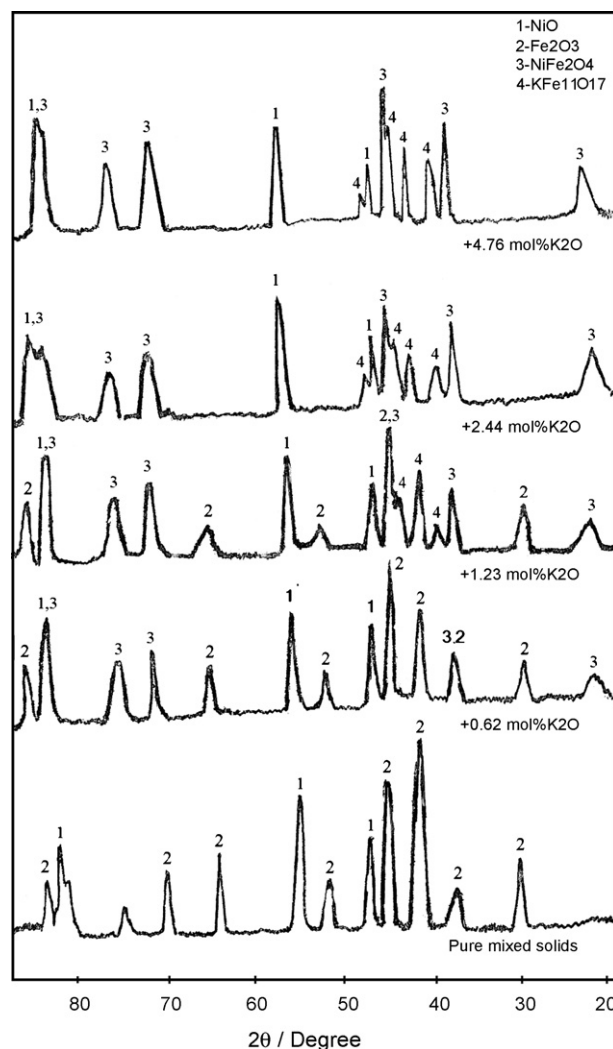
Fig. 4. X-ray diffractograms of pure mixed solids and that doped with different amounts of K_2O followed by calcination at 750^\circ C .
