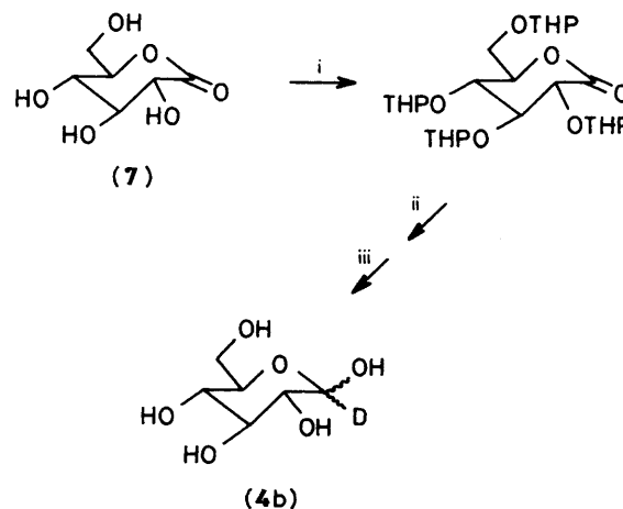
Scheme 2. Reagents: i, DHP-TsOH-DMF; ii, \text{LiAlD}_4-\text{AlCl}_3-\text{Et}_2\text{O} ; iii, Dowex 50Wx4
