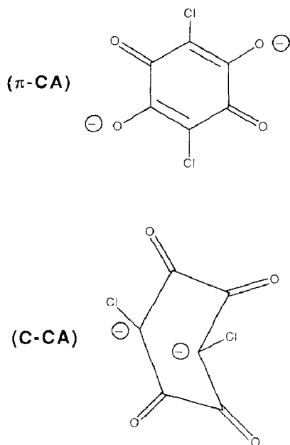
Fig. 1. Chloranilate C-CA 2- and π-CA 2- ligands.
