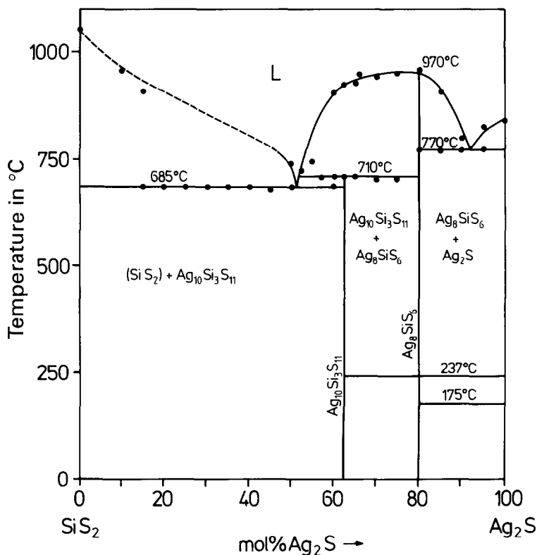
Fig. 2. Phase diagram of the \text{Ag}_2\text{S} - \text{SiS}_2 system.
