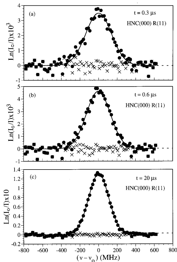
Figure 1. Absorption line profiles for R(11) of the HNC(10 0 0) \leftarrow HNC(00 0 0) transition obtained at various observation times following the initiation of reaction 2b. The solid lines are Gaussian frequency profiles fit to the data, and the residues are indicated by the crosses. At a delay time of 20 \mu s, Panel (c), the HNC product had equilibrated to the temperature of the reaction chamber, 293 K. The conditions of the experiment were P_{\text{CH}_3\text{SH}} = 0.050 and P_{\text{CN}_2} = 0.050 Torr for a KrF laser energy of 300 mJ/pulse. At 293 K, the Doppler width for the R(11) transition is 262 MHz.
