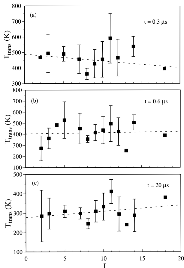
Figure 8. Similar to Figure 7 except for the HNC(01 1 0) vibrational level.
