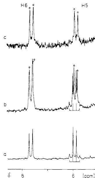
Figure 1. 1 H NMR spectra (H5, H6 resonances only) of cis\text{-}[(NH_3)_2PtC_2]Cl_2 (0.025 M): (a) immediately after addition of CN − (0.5 M, D 2 O, pD 8.3); (b) after 12 h at 30 °C (Approximately 50% of the bound C is replaced. The spectrum consists of signals due to starting compound and free C (circles)); (c) after 50 h at 30 °C (At that stage, the solution contains some precipitate of cis\text{-}[(NH_3)_2PtC_2][Pt(CN)_4] (cf. text)).
