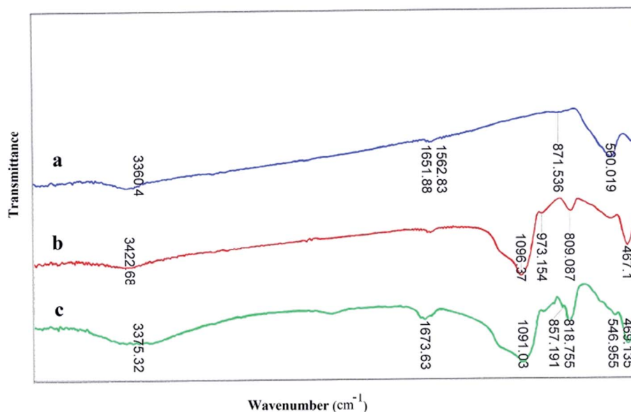
Fig. 1 The comparative FT-IR spectra of (a) \text{Fe}_3\text{O}_4 NPs (b) \text{Fe}_3\text{O}_4\text{@SiO}_2 and (c) \text{Fe}_3\text{O}_4\text{@SiO}_2\text{-MoO}_3\text{H} .
