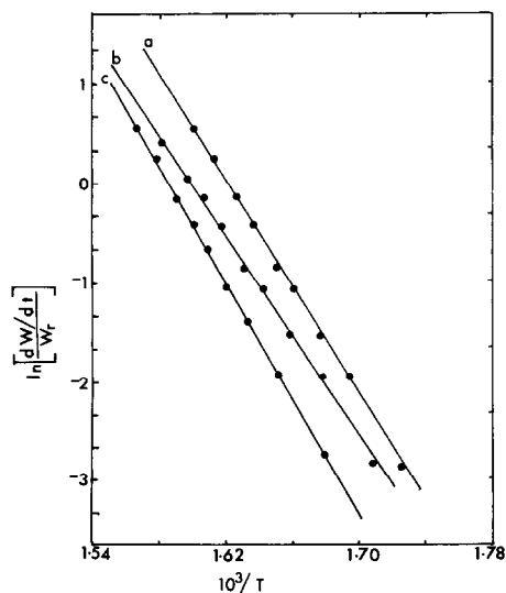
Fig. 4. Freeman-Carroll plot for a = \text{Ni(L)} \cdot \text{H}_2\text{O} , b = \text{Zn(L)} \cdot \text{H}_2\text{O} and c = \text{Cd(L)} .
