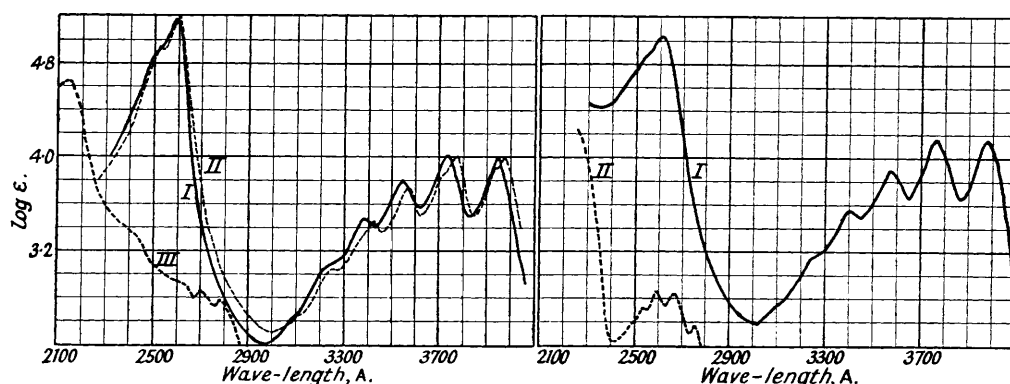
FIG. 1.—I, 9-Methyl-10-ethoxymethylanthracene (in alcohol). Max. (and log \epsilon ) at 2520 (4.93), 2590 (5.24), (3100, 2.69), (3250, 3.08), 3390 (3.48), 3550 (3.80), 3740 (4.01), (3870, 3.71), and 3950 (3.98). II, 9 : 10-Dimethylanthracene (after Jones, J. Amer. Chem. Soc., 1945, 67, 2127). III, 9-Methyl-10-ethoxymethylanthracene photo-oxide (in alcohol).
