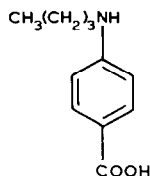
4-(butylamino) benzoic acid ( \text{C}_{11}\text{H}_{15}\text{NO}_2 )
